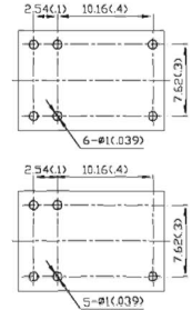
Drilling Plan孔位图 (Bottom View/底视图)
